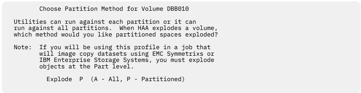
Figure 57. Specifying partition processing
