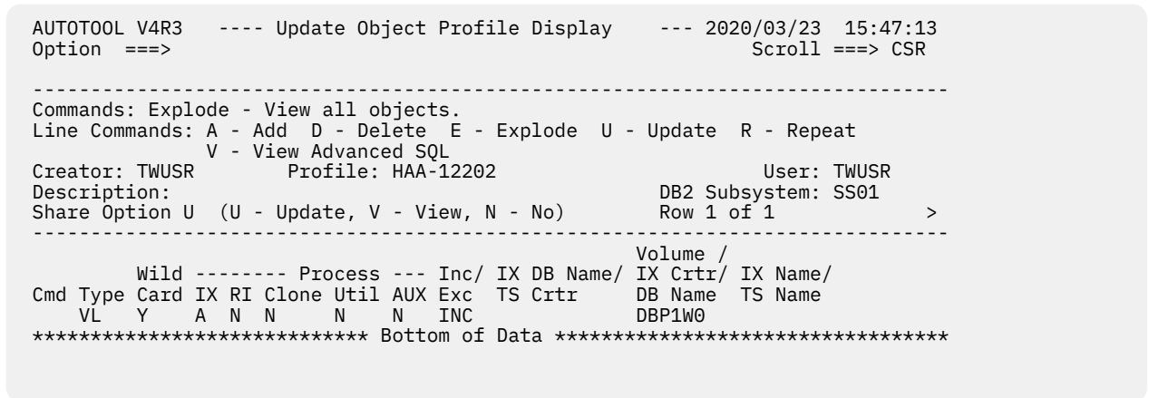
Figure 58. Update Object Profile Display
