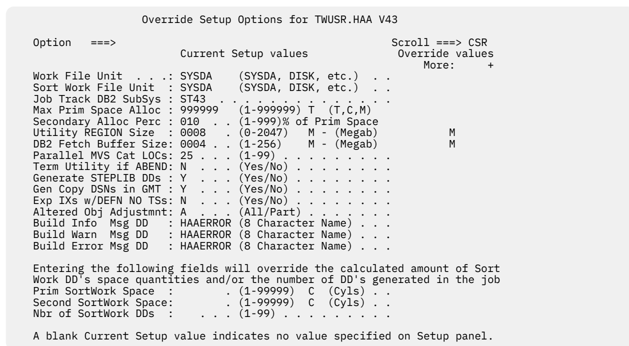
Figure 177. Override Setup Options window
